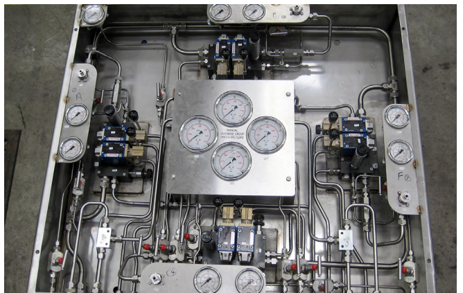
Control panel pipework installation
